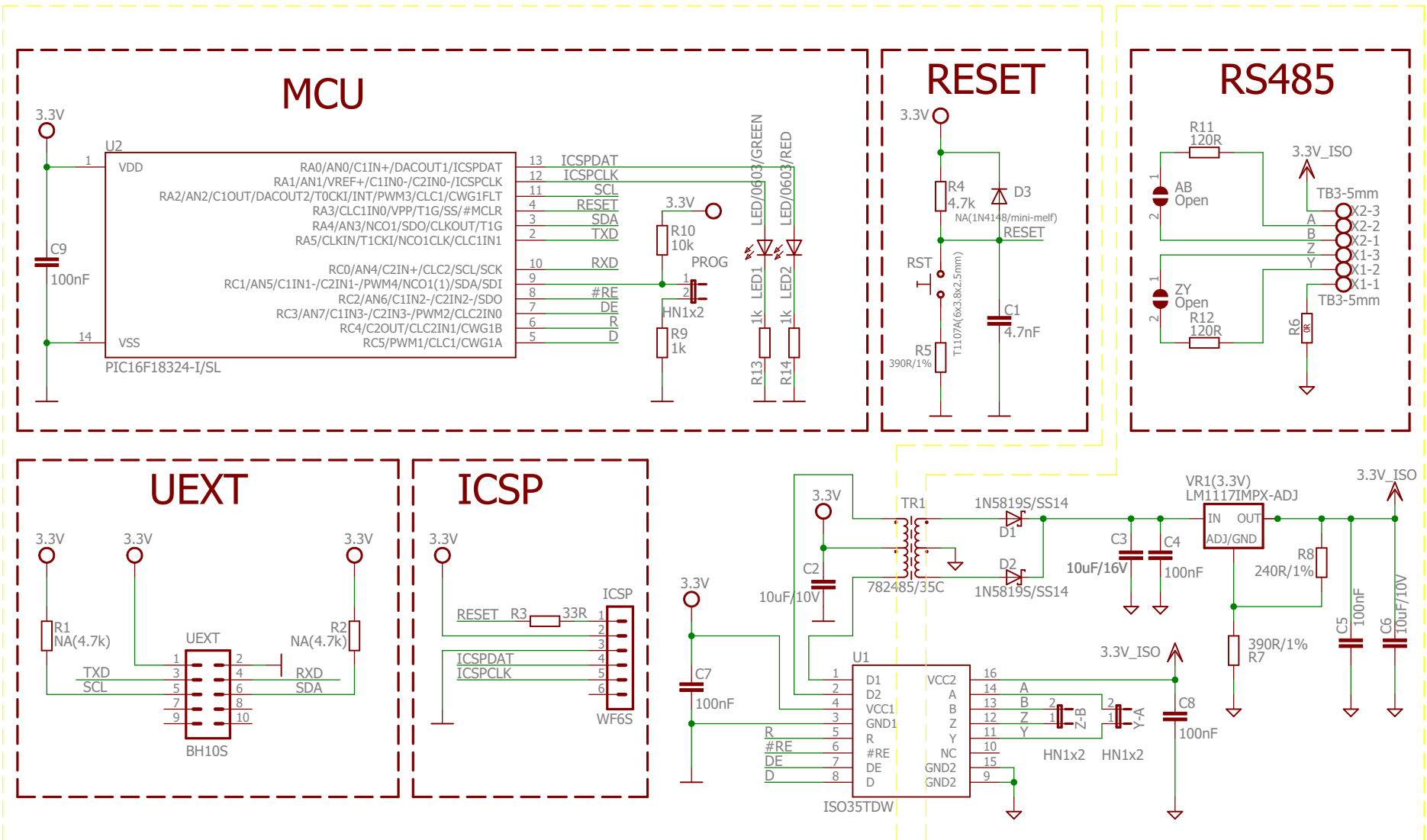
MOD-RS485-ISO, hardware revision C
